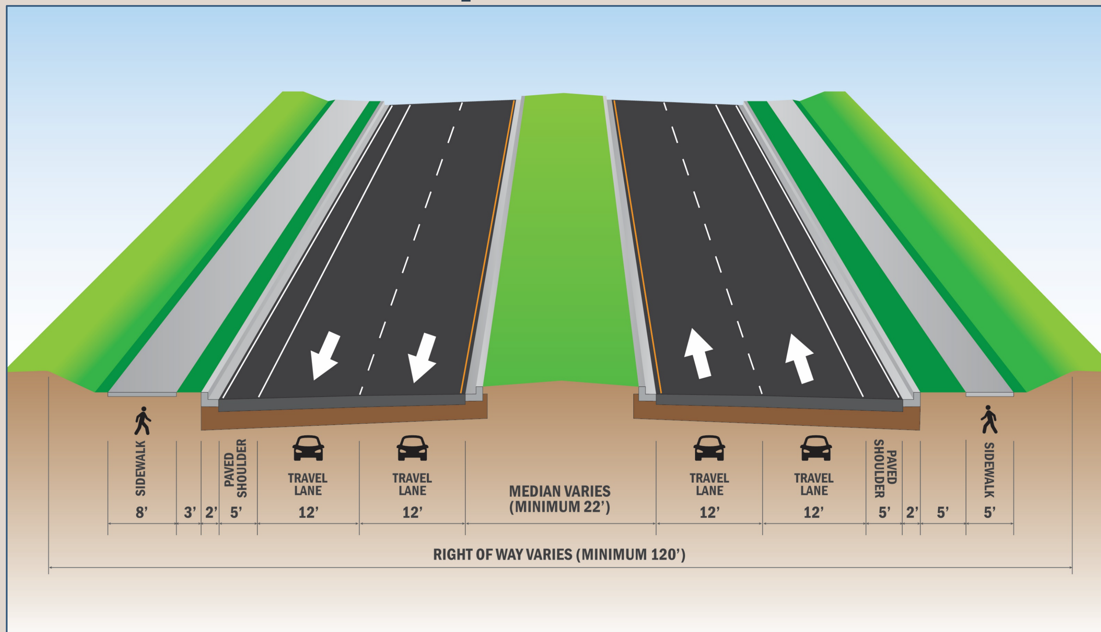
Proposed Road
