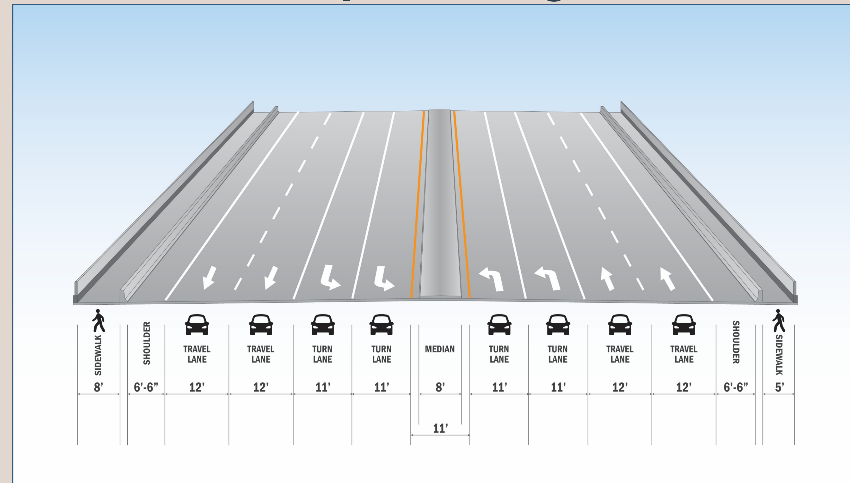
Proposed Bridge
