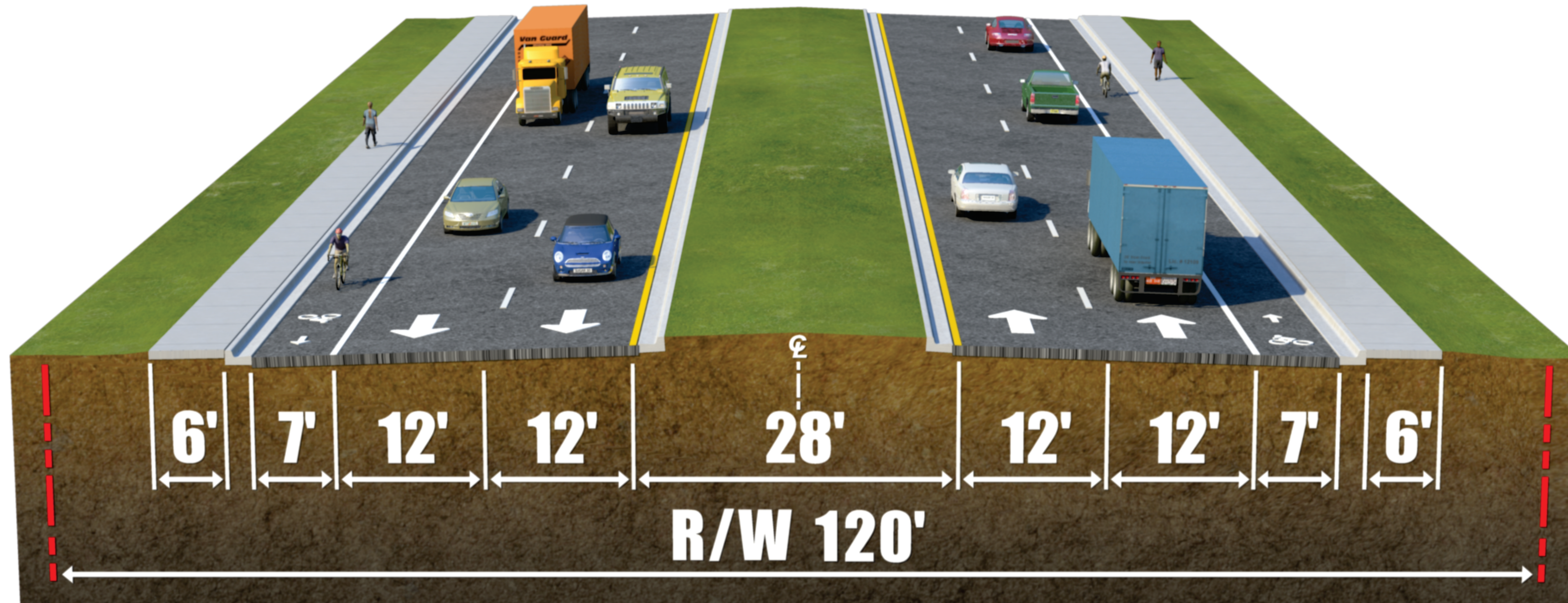
NW 49 th Street Proposed Typical Section Posted Speed Limit: 45 mph
