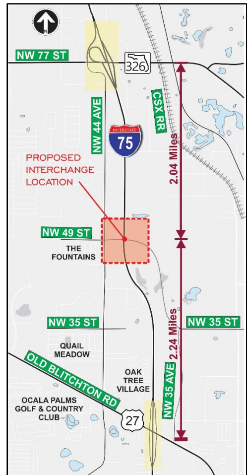
Figure 2-3 - Existing Interchanges
