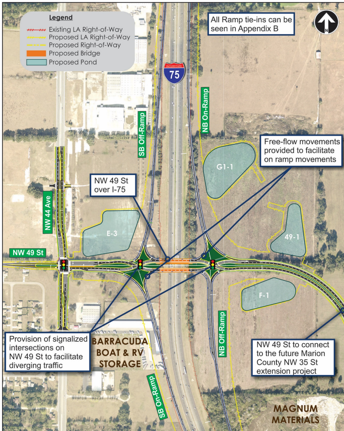
Figure 6-1 - Preferred Alternative
