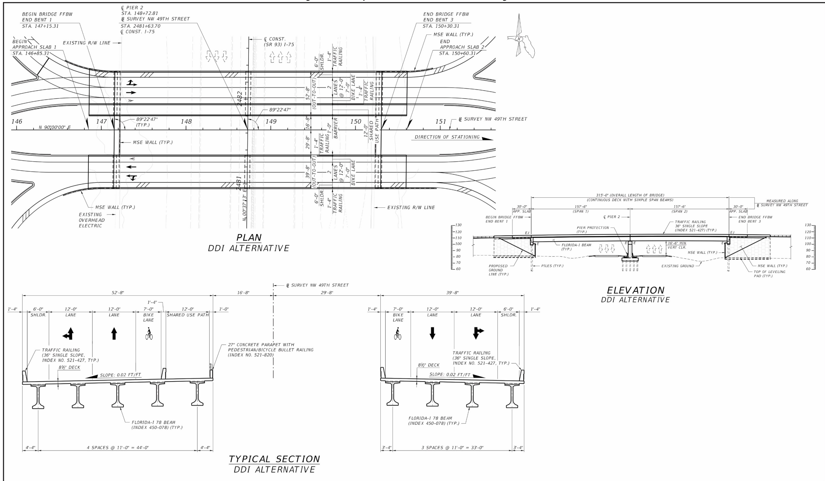
Figure 6-3 - Proposed NW 49 Street over I-75 Bridge Characteristics
