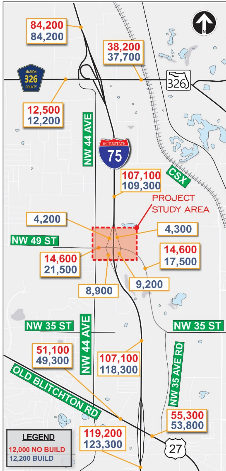
Figure 4-2 - 2045 AADT
