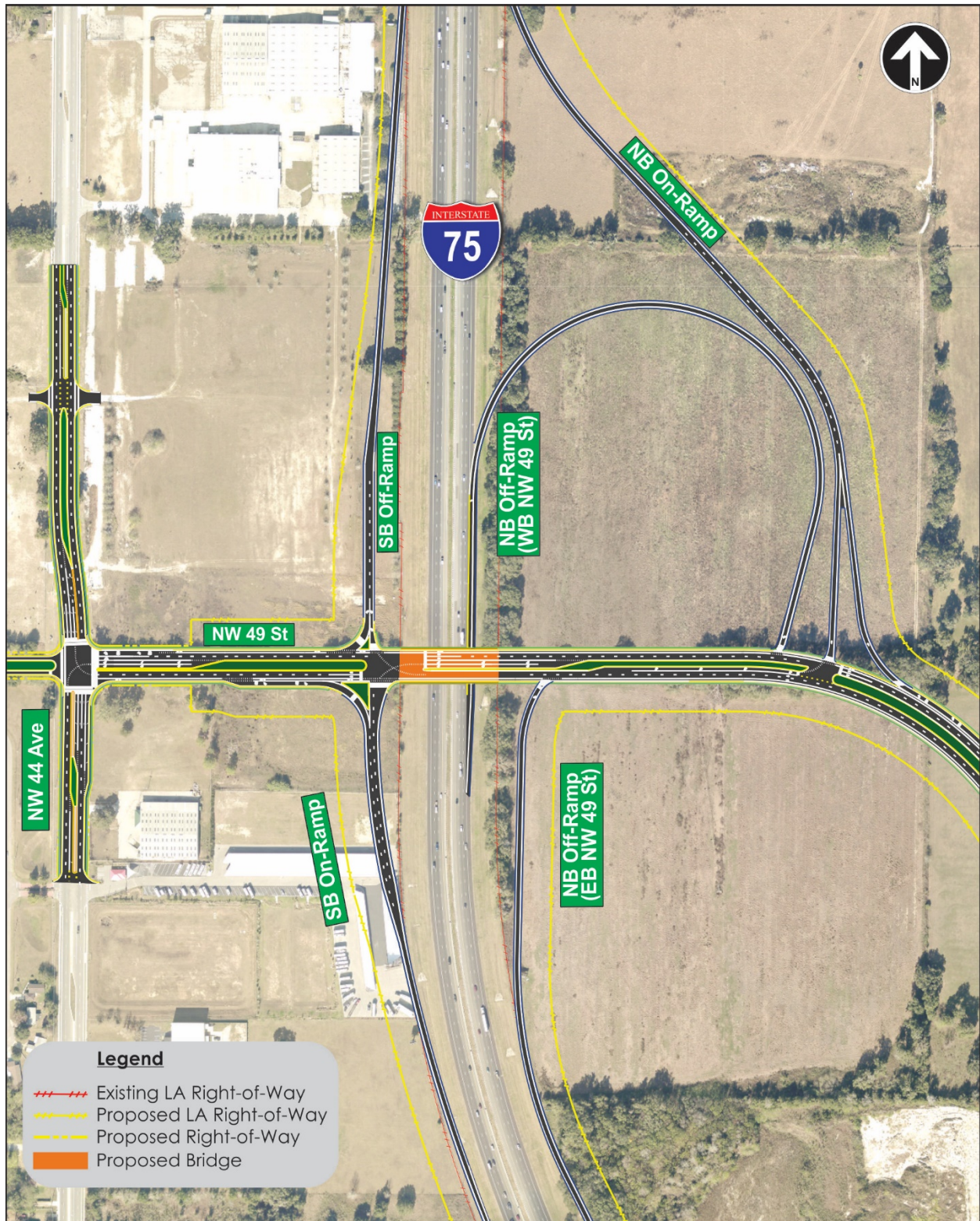
Figure 4-8 - Preliminary Parclo NE Interchange
