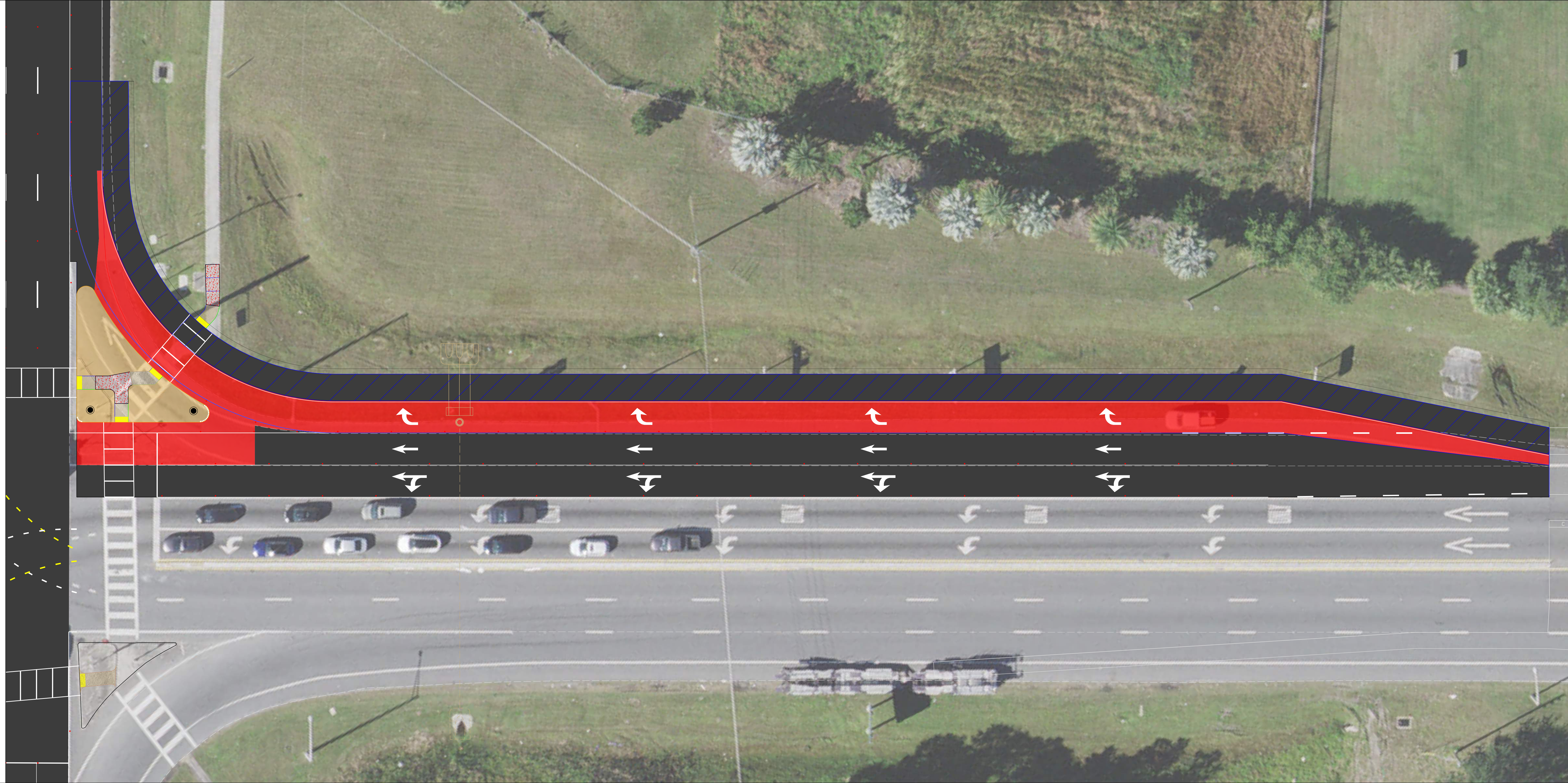
FLORIDA'S TURNPIKE ACCESS DETAIL
