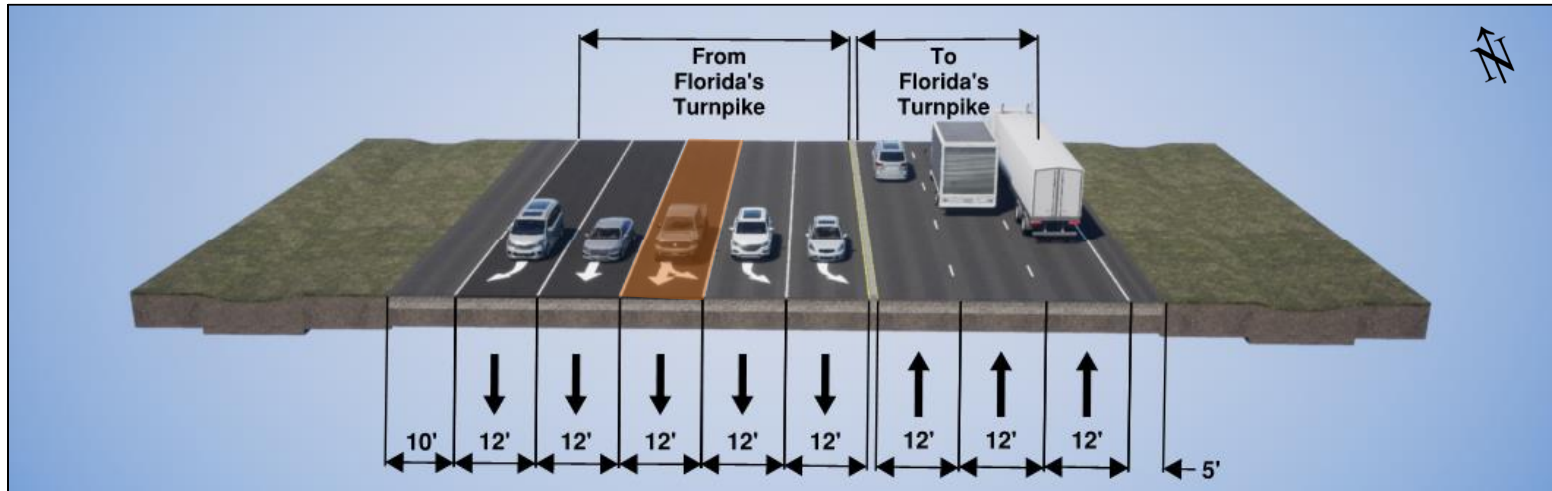
Typical Section 3: Florida's Turnpike Access Road
