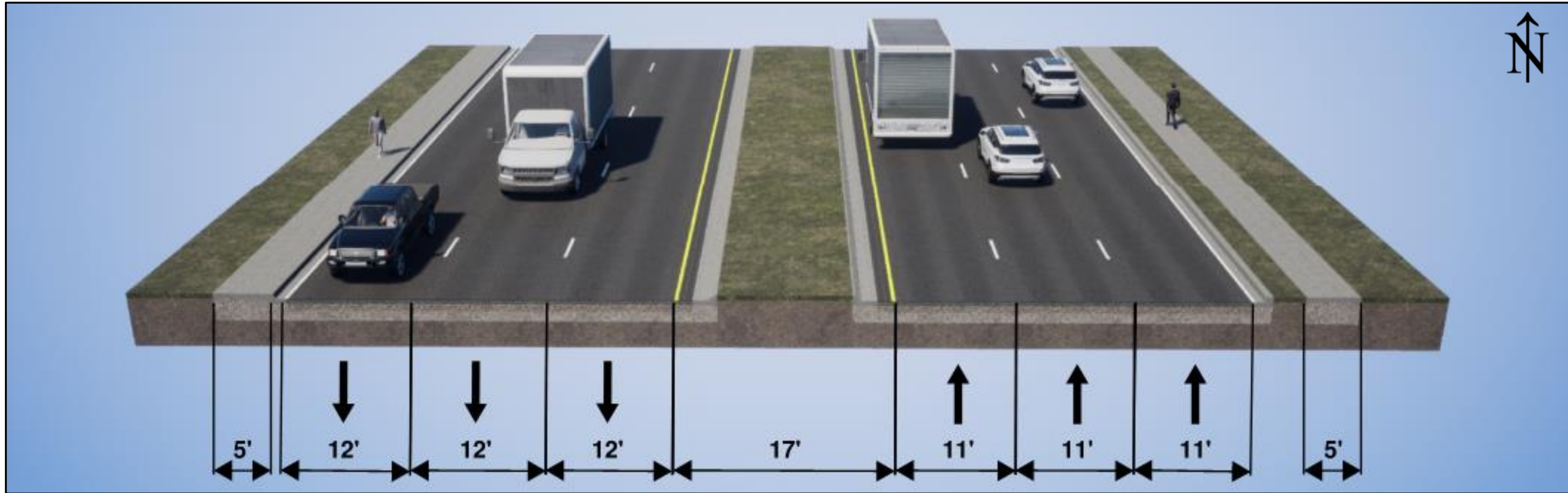
Typical Section 1: U.S. 192 from Main St to Michigan Ave
