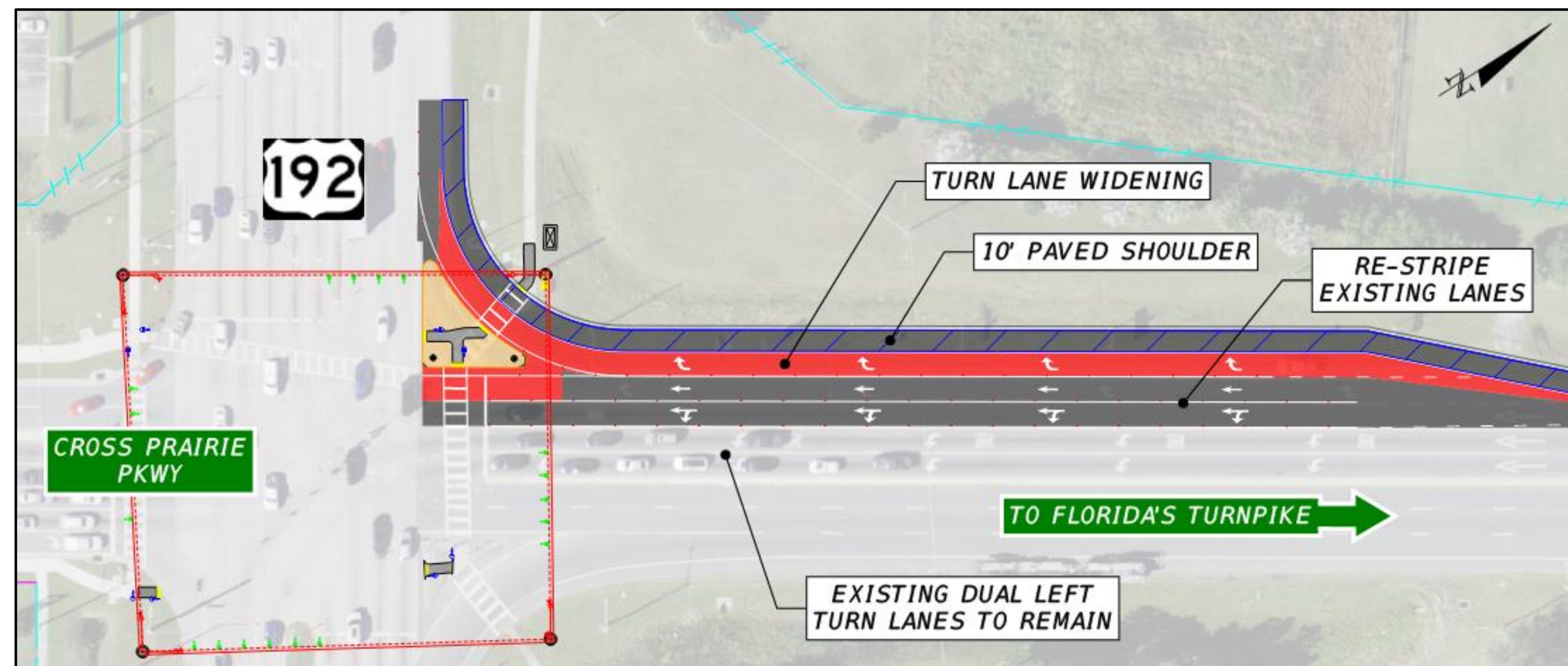
Florida's Turnpike Access Road Improvements
