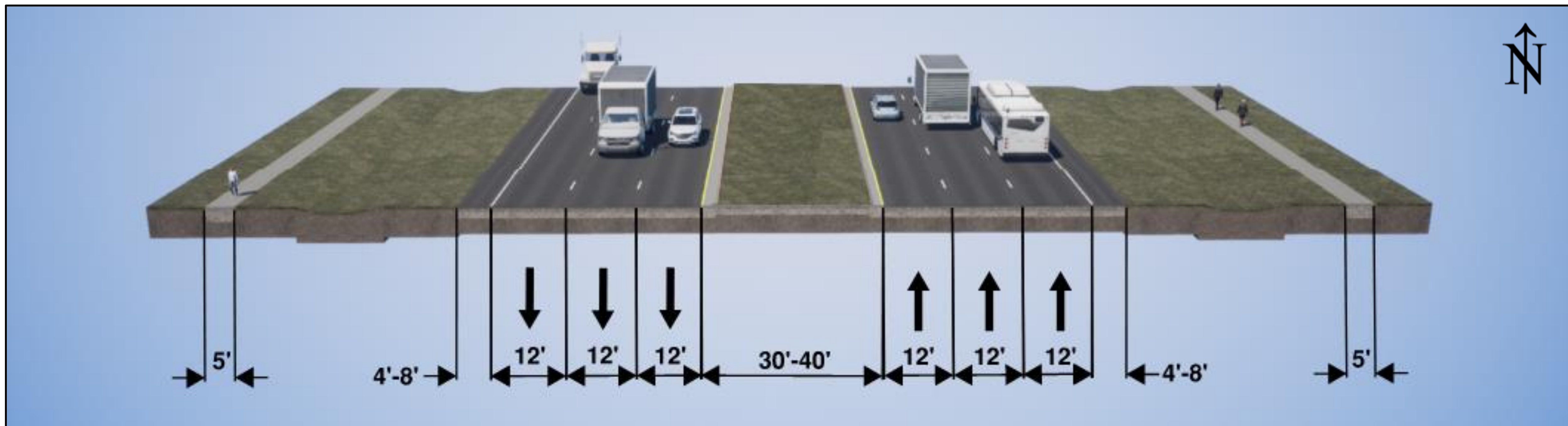
Typical Section 2: U.S. 192 from to Michigan Ave to Aeronautical Dr
