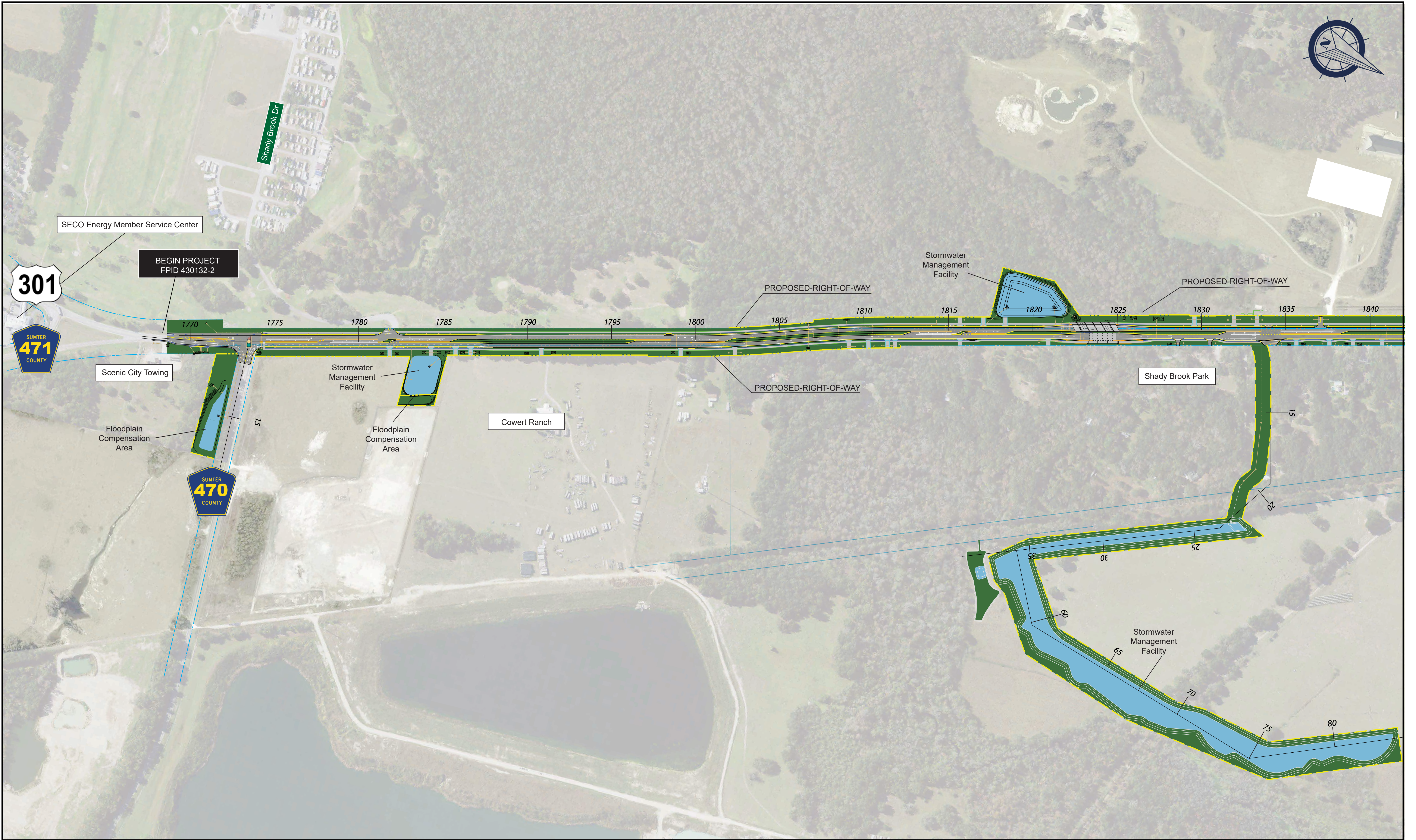
U.S. 301 (S.R. 35) Improvements U.S. 301 Widening C.R. 470 to Industrial Park Drive (C.R. 525E) (FPID #430132-2)
