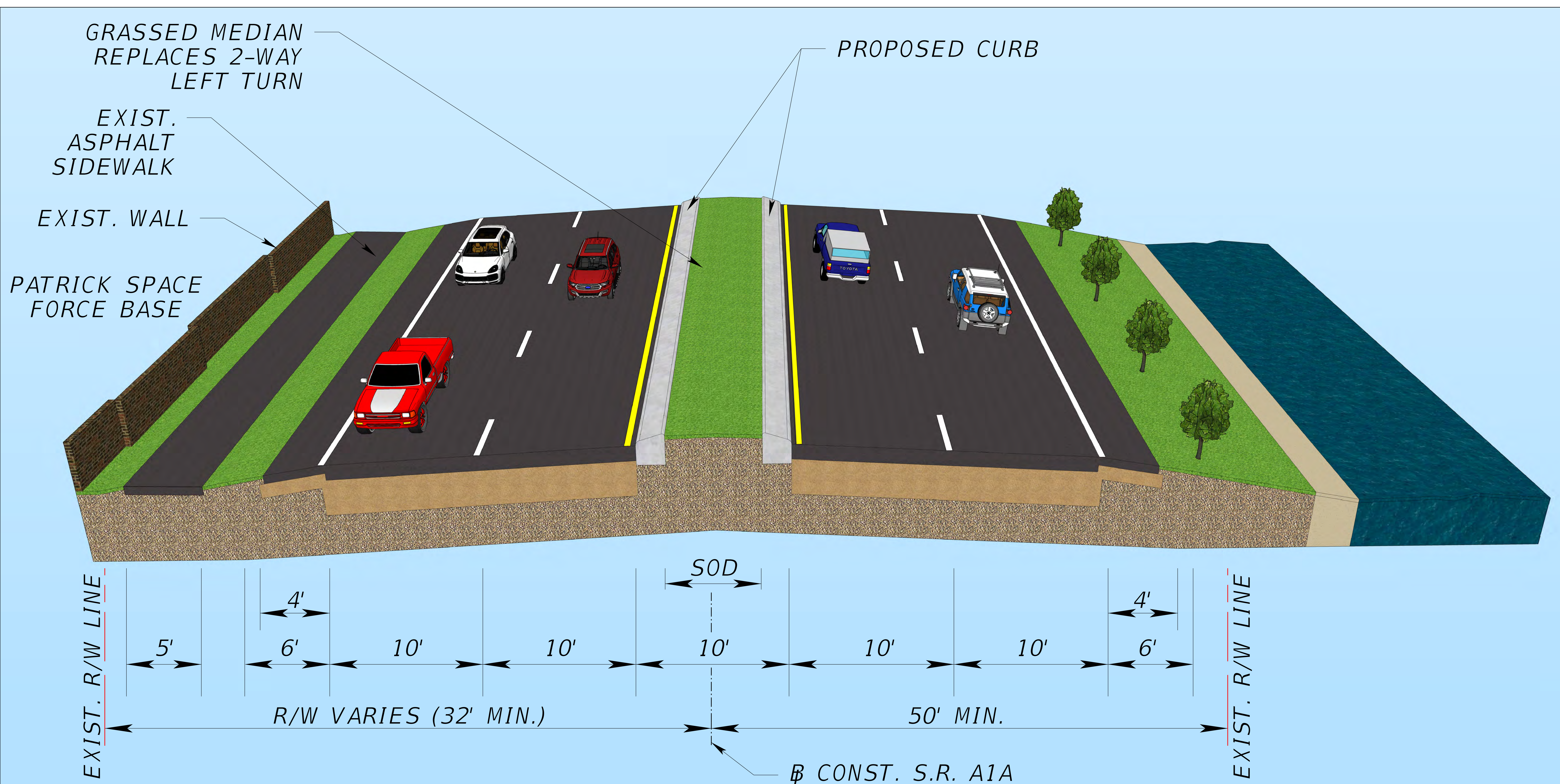
PROPOSED TYPICAL SECTION NO. 1 FROM NORTH OF PINEDA CAUSEWAY TO SOUTH OF SCHOOL AVENUE APPROXIMATE SEGMENT LENGTH: 0.7 MILES
