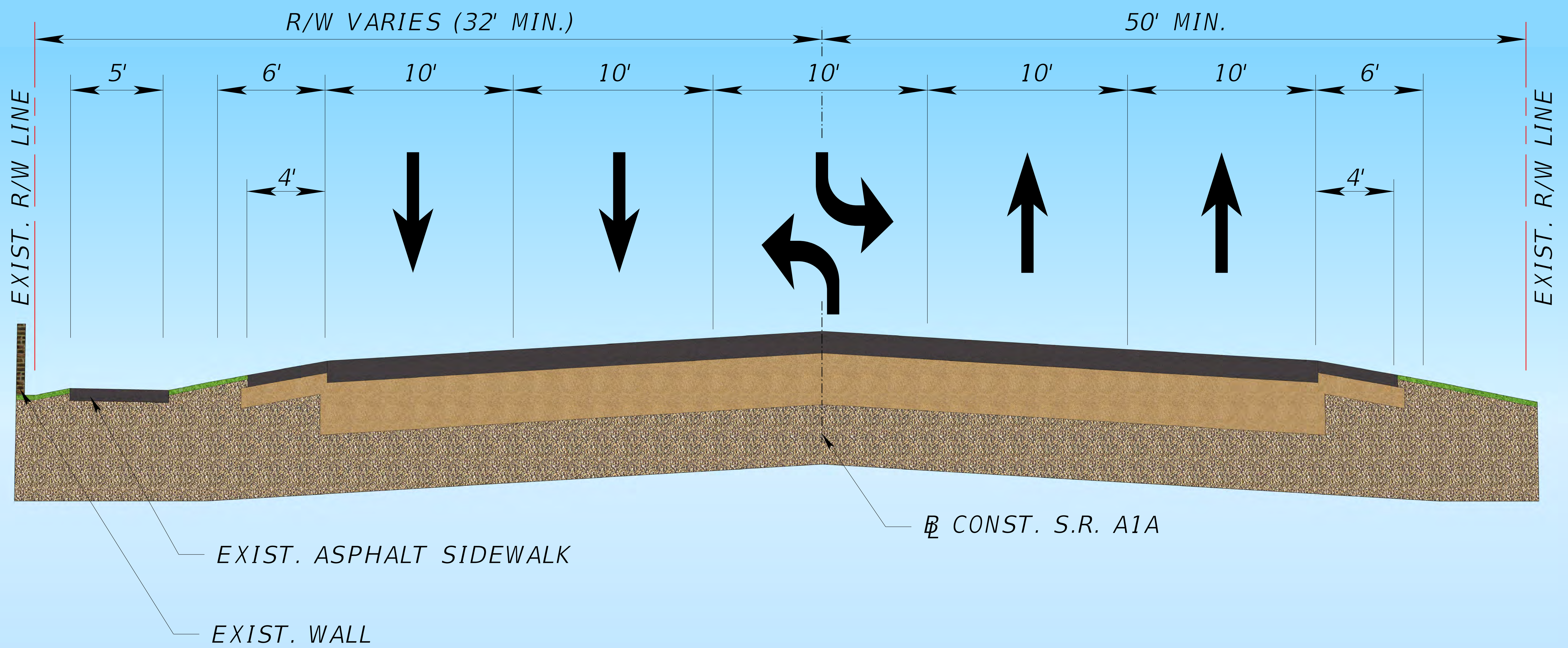
EXISTING TYPICAL SECTION NO. 1 FROM NORTH OF PINEDA CAUSEWAY TO SOUTH OF SCHOOL AVENUE APPROXIMATE SEGMENT LENGTH: 0.7 MILES
