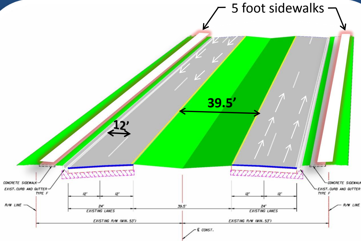
TYPICAL SECTION SR 600 (JOHN YOUNG PARKWAY) EXISTING CONDITION
