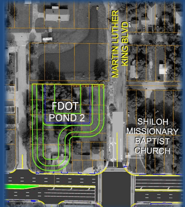
FDOT Pond 2
