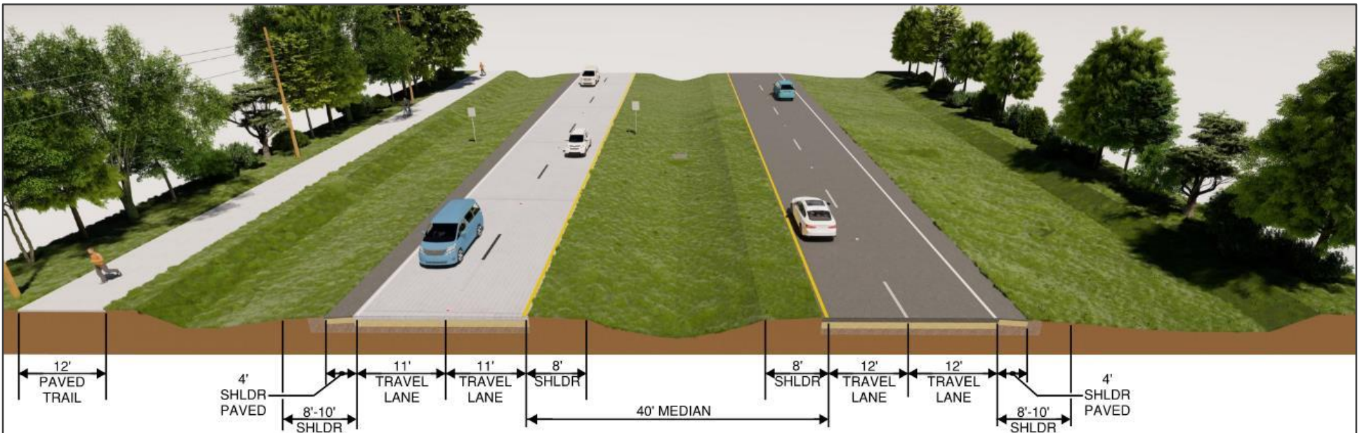
Proposed Typical Section From North Garfield Avenue to east of North Kepler Road
