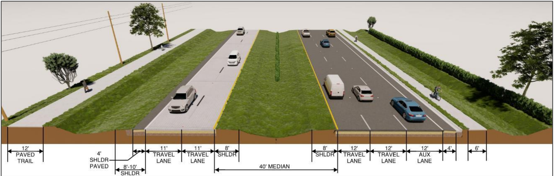
Proposed Typical Section East of Alabama Avenue to North Garfield Avenue
