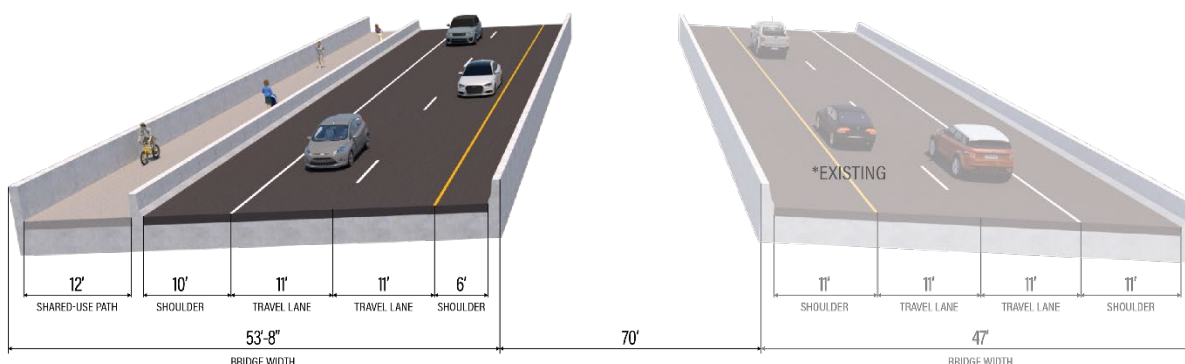
Figure 6: Bridge Typical Section (Segment 2)
