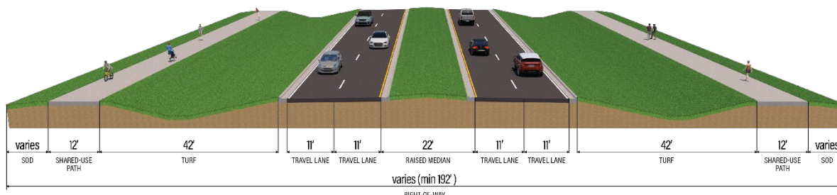
Figure 5: Suburban Typical Section (Segments 1, 4, and 6)
