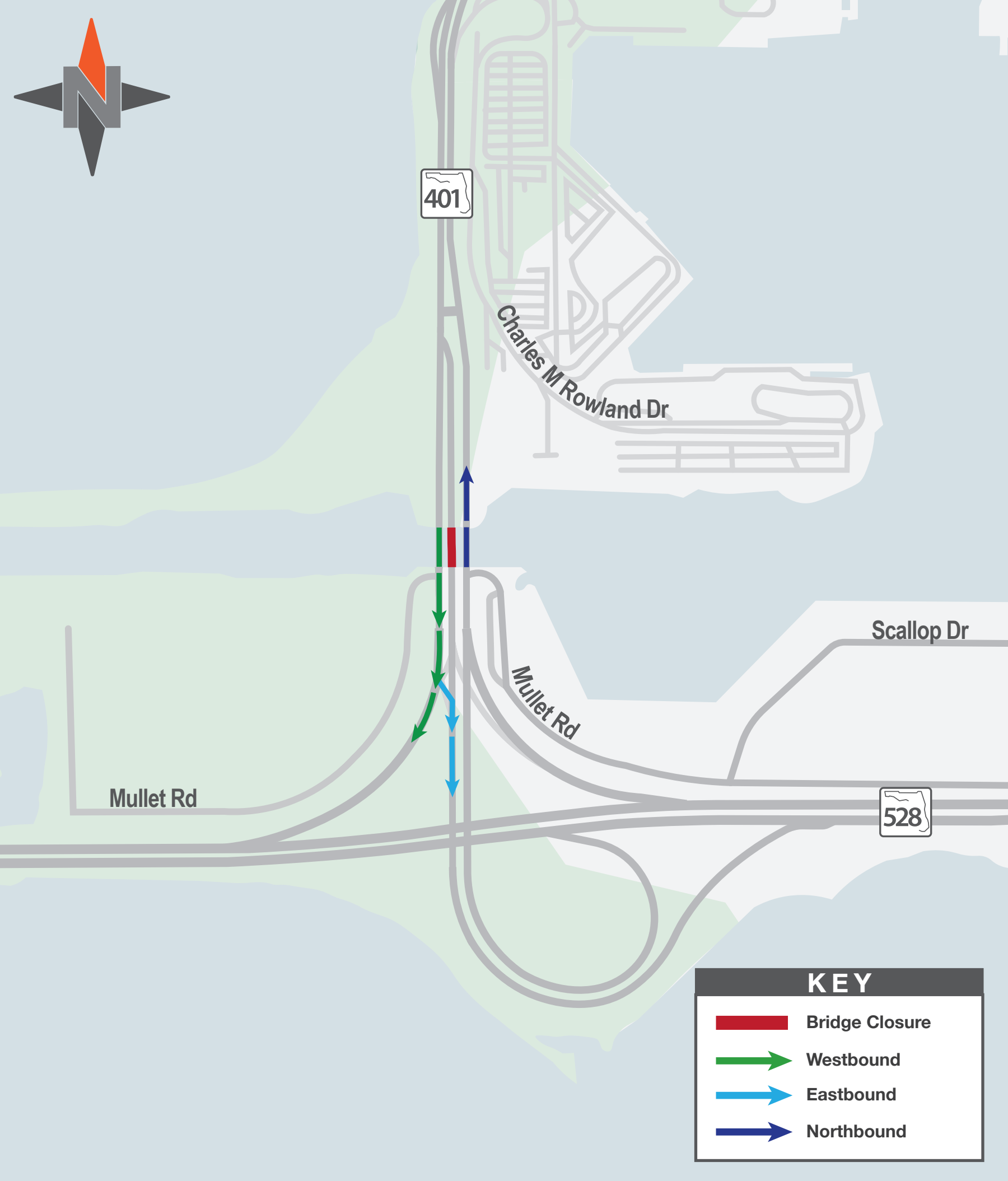
EB S.R. 401 Bridge Detour
