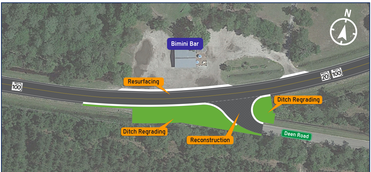
Figure 1: Proposed Intersection Improvements at S.R. 100 and Deen Road.
