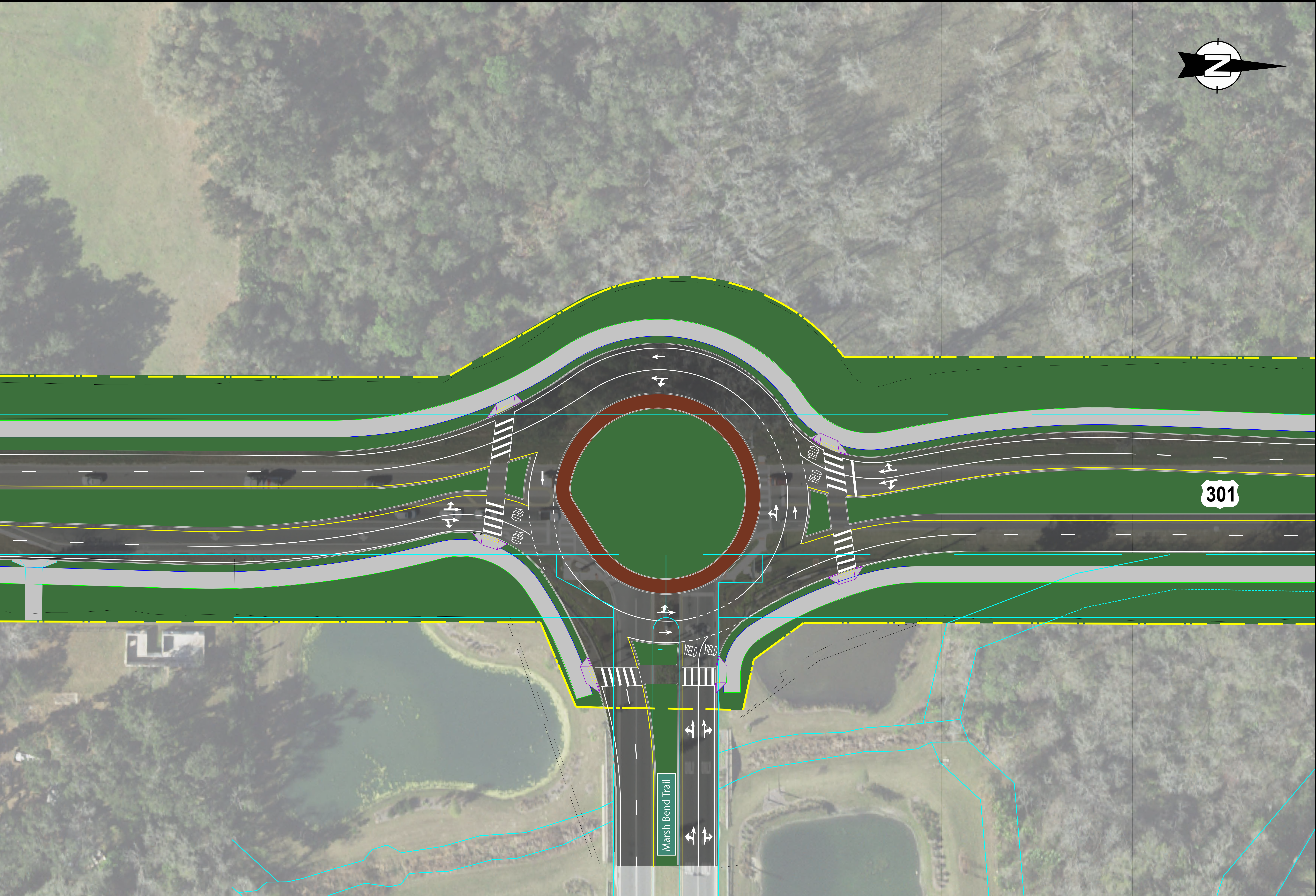
U.S. 301 (S.R. 35) Improvements U.S. 301 Realignment from Warm Springs Avenue to Florida's Turnpike (FPID #430132-5 & 430132-4 Interchange Improvements)
