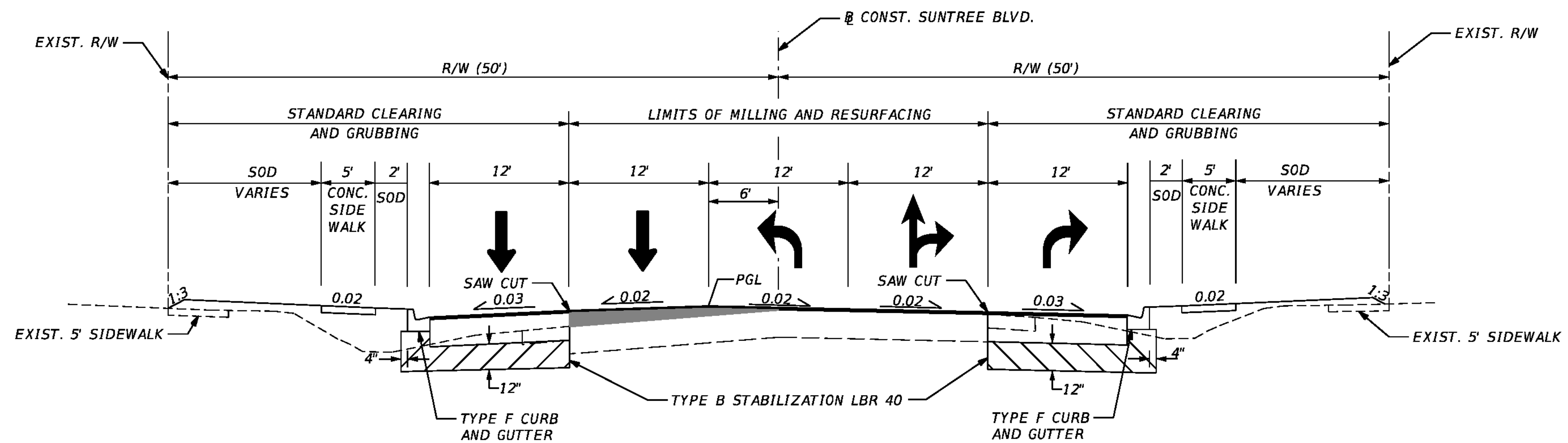
Suntree Boulevard – Proposed Typical Section
