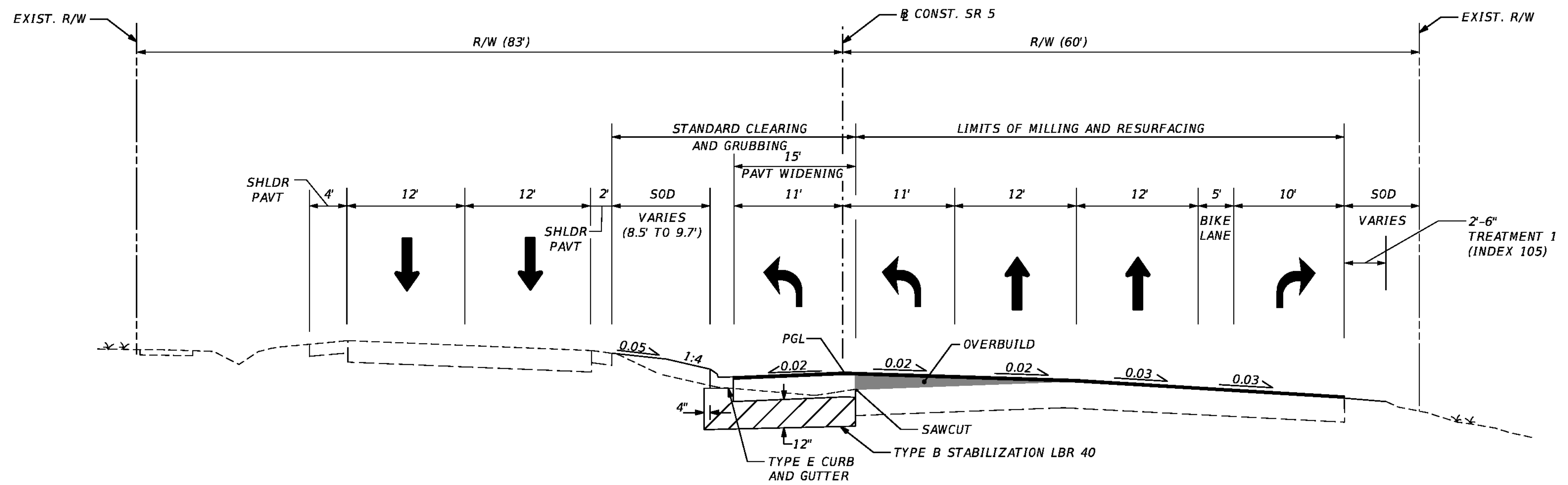
State Road (S.R.) 5/U.S. 1 – Proposed Typical Section
