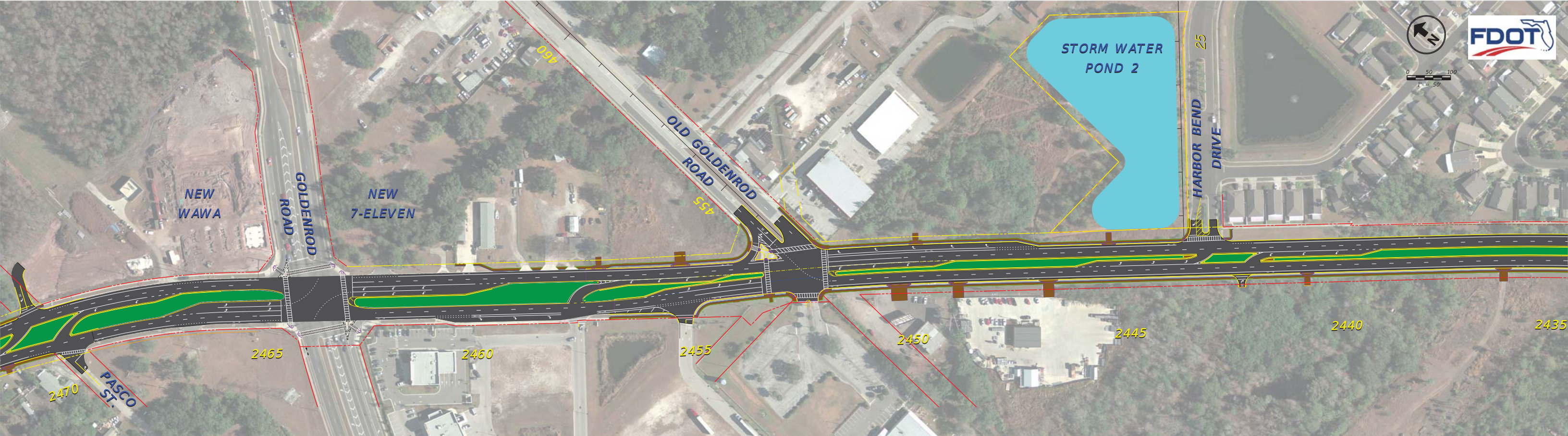
SR 15 (Hoffner Avenue) Widening 239266-3-52-01 & 239266-4-52-01 From Lee Vista Boulevard to Conway Road
