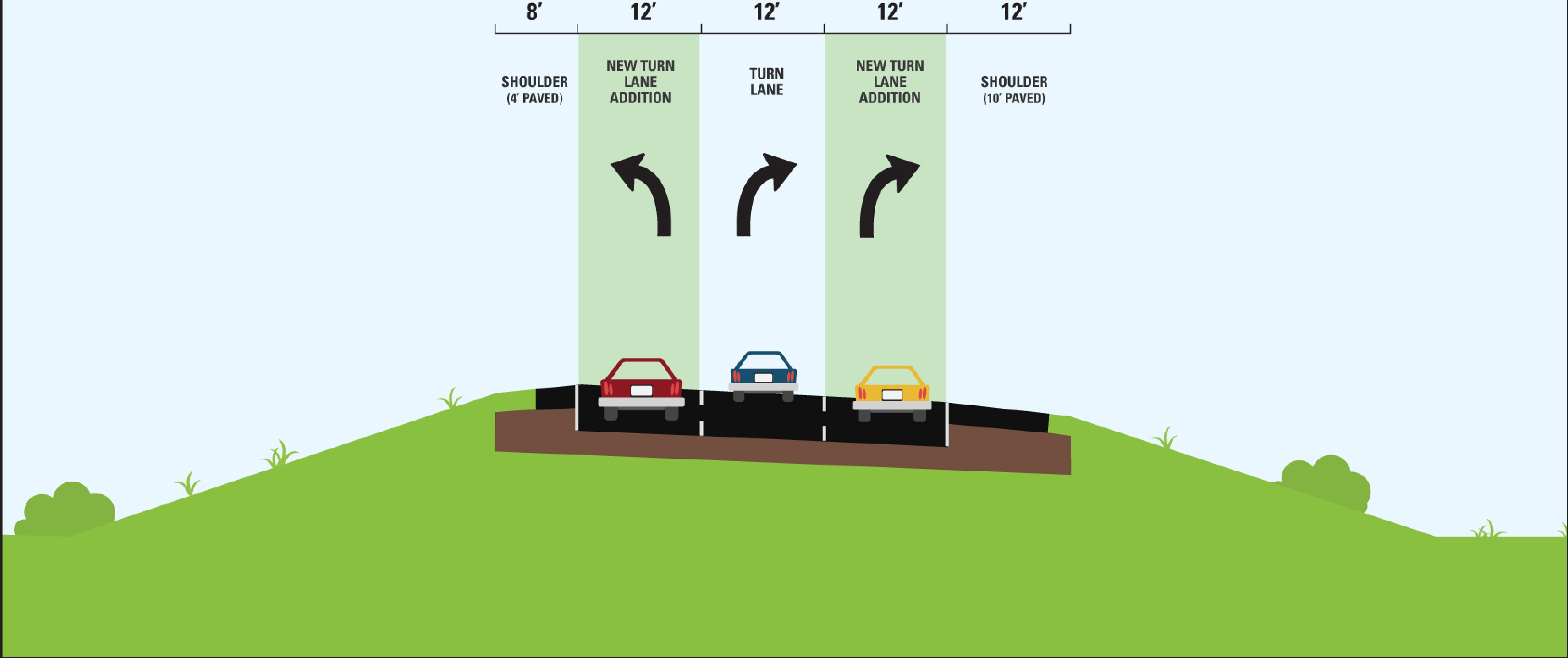
Proposed Typical Section Northbound I-95 Off Ramp to S.R. 518
