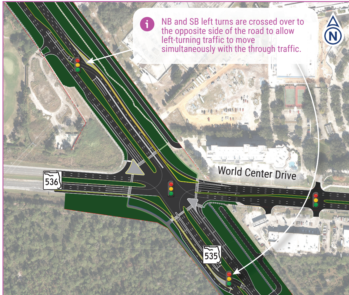
Option A: Displaced Left Intersection
