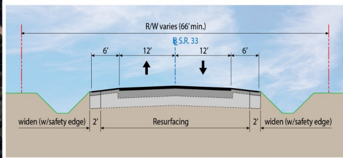
ROADWAY TYPICAL SECTION
