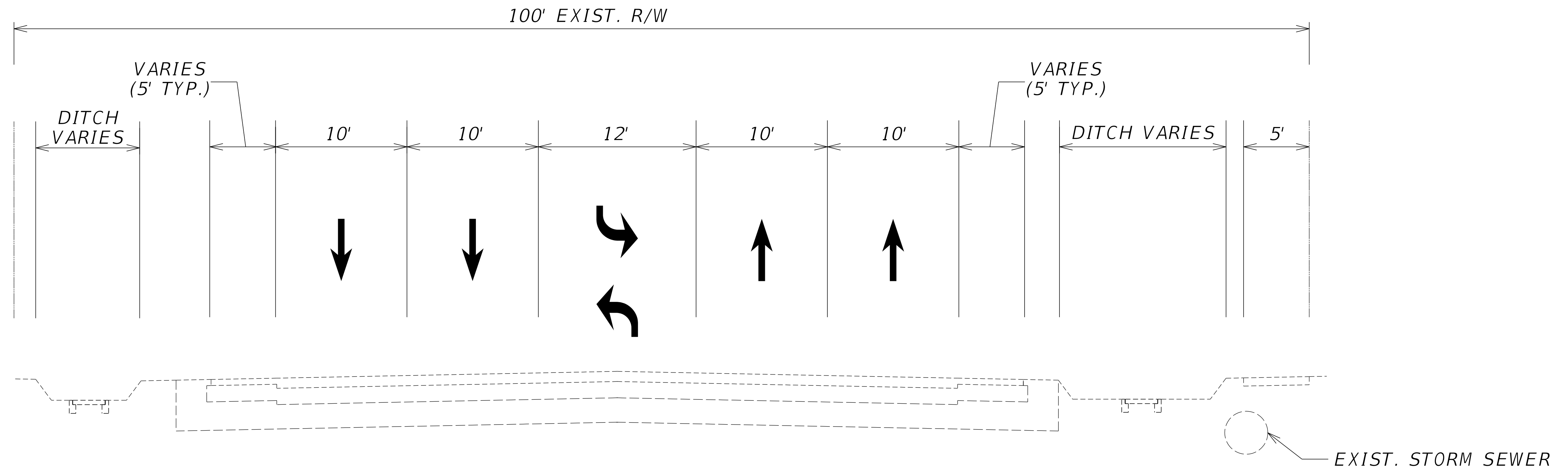
EXISTING TYPICAL SECTION
